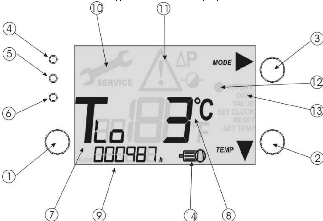
Illustration 3: Control keypad with status displays
